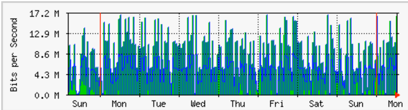
GSFC-McLean 10 GigE "Lambda49" across DRAGON: 'Weekly' (30 Minute Averages) 21 November 2005
